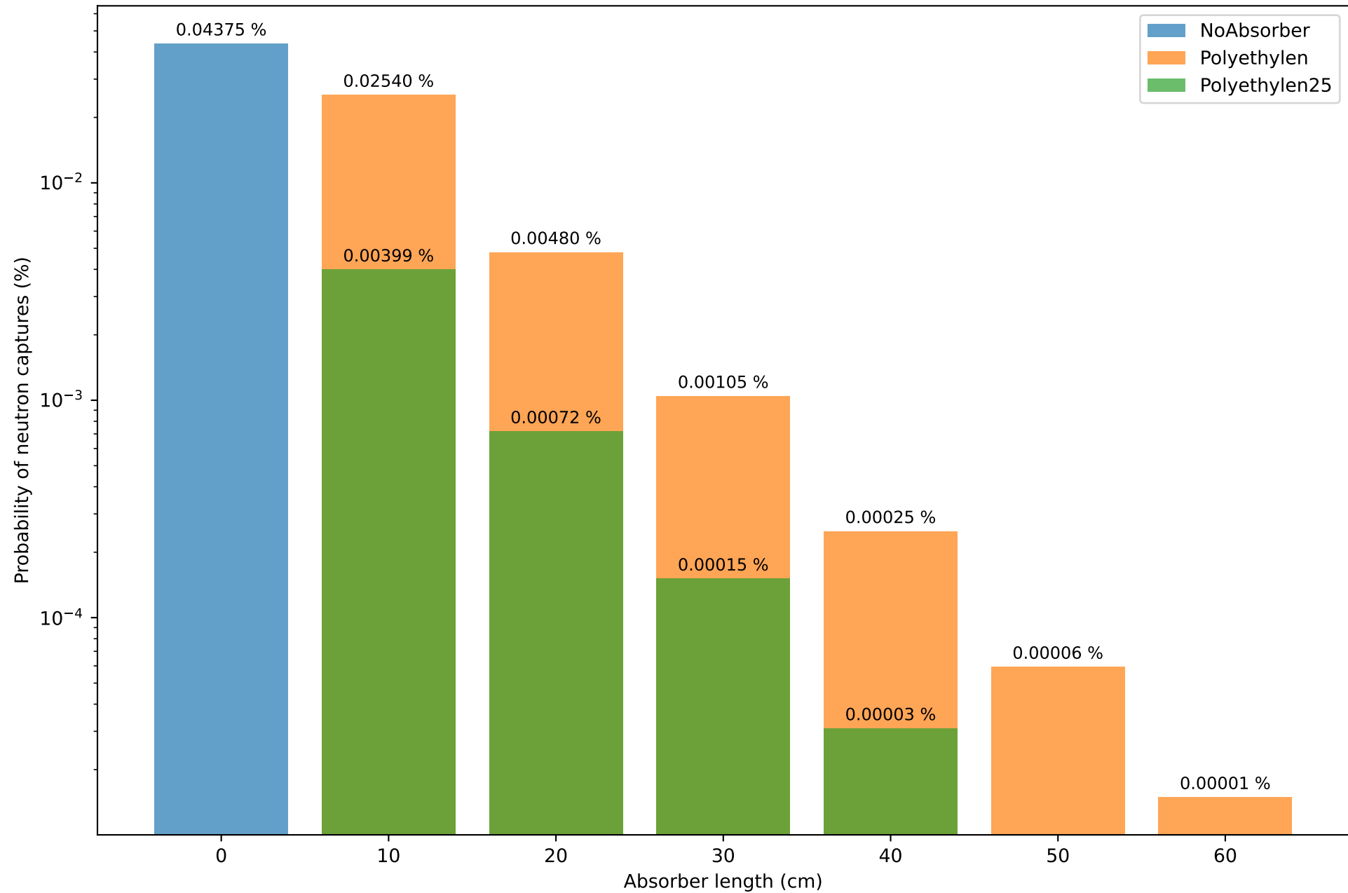
Neutron captures probabilities in LXe with different absorber and lengths
