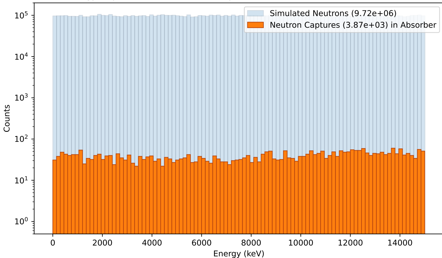
Energy dependence of Neutron Captures in the 5cm Paraffin25 Absorber
