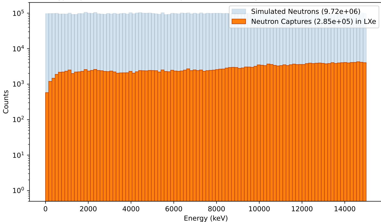
Energy dependence of Neutron Captures in LXe using a 5cm Paraffin25 Absorber
