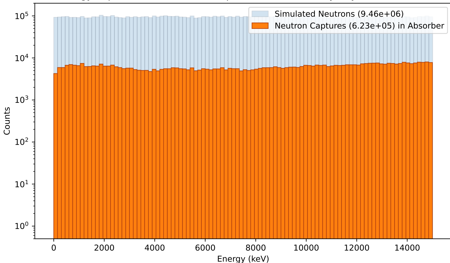
Energy dependence of Neutron Captures in the 5cm Polyethylene Absorber
