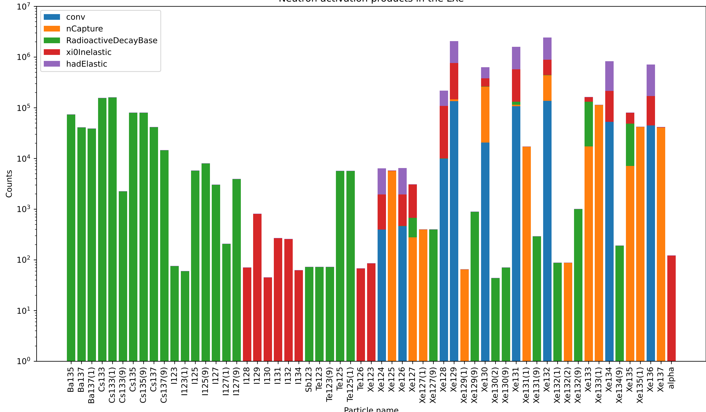
Neutron activation products in the LXe
