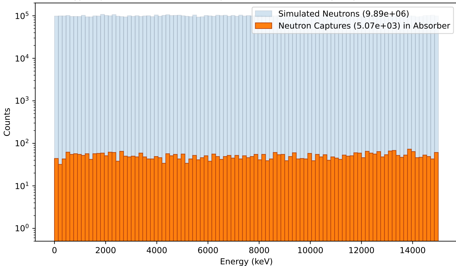
Energy dependence of Neutron Captures in the 15cm Polyethylene25 Absorber
