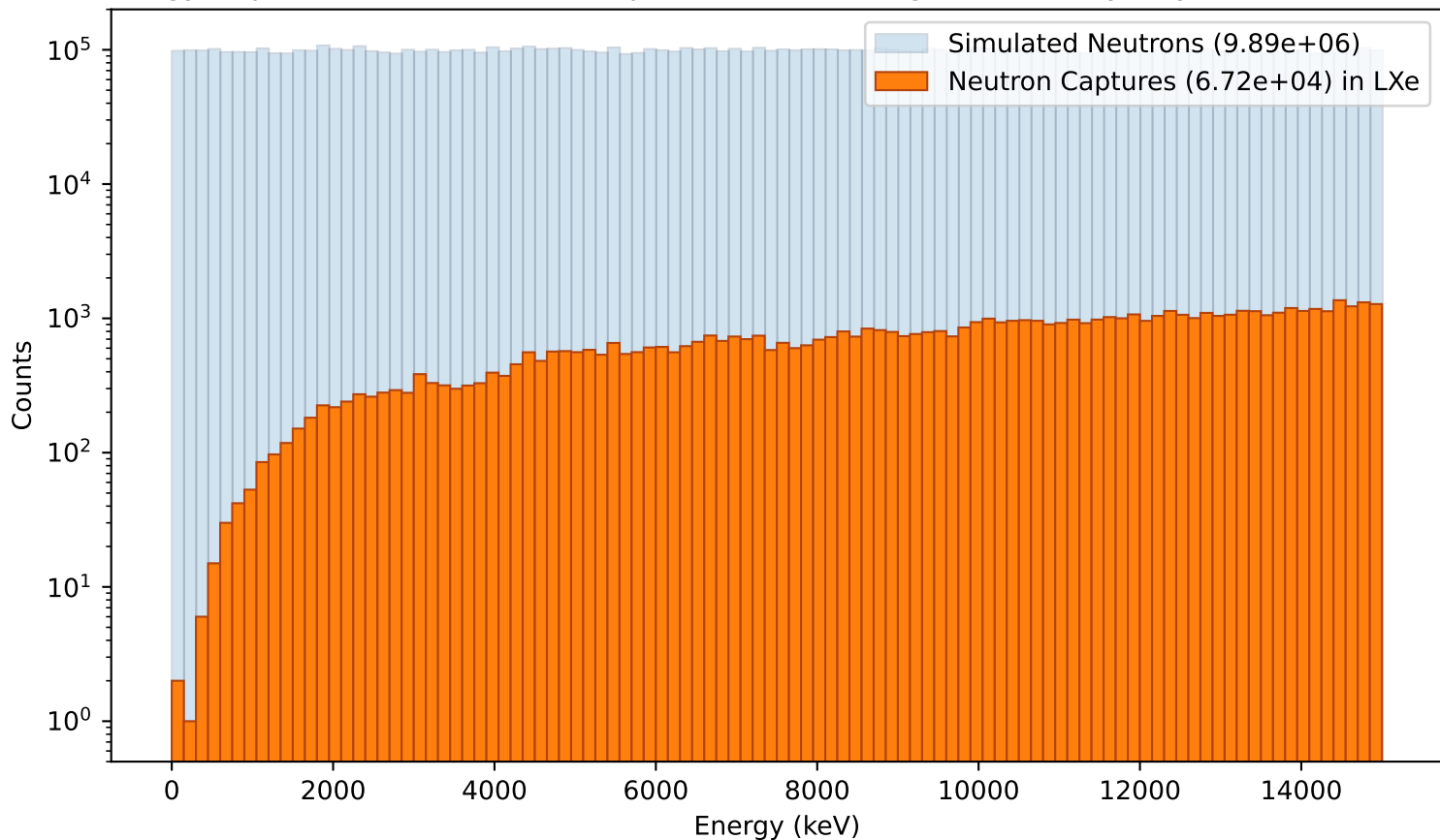
Energy dependence of Neutron Captures in LXe using a 15cm Polyethylene25 Absorber
