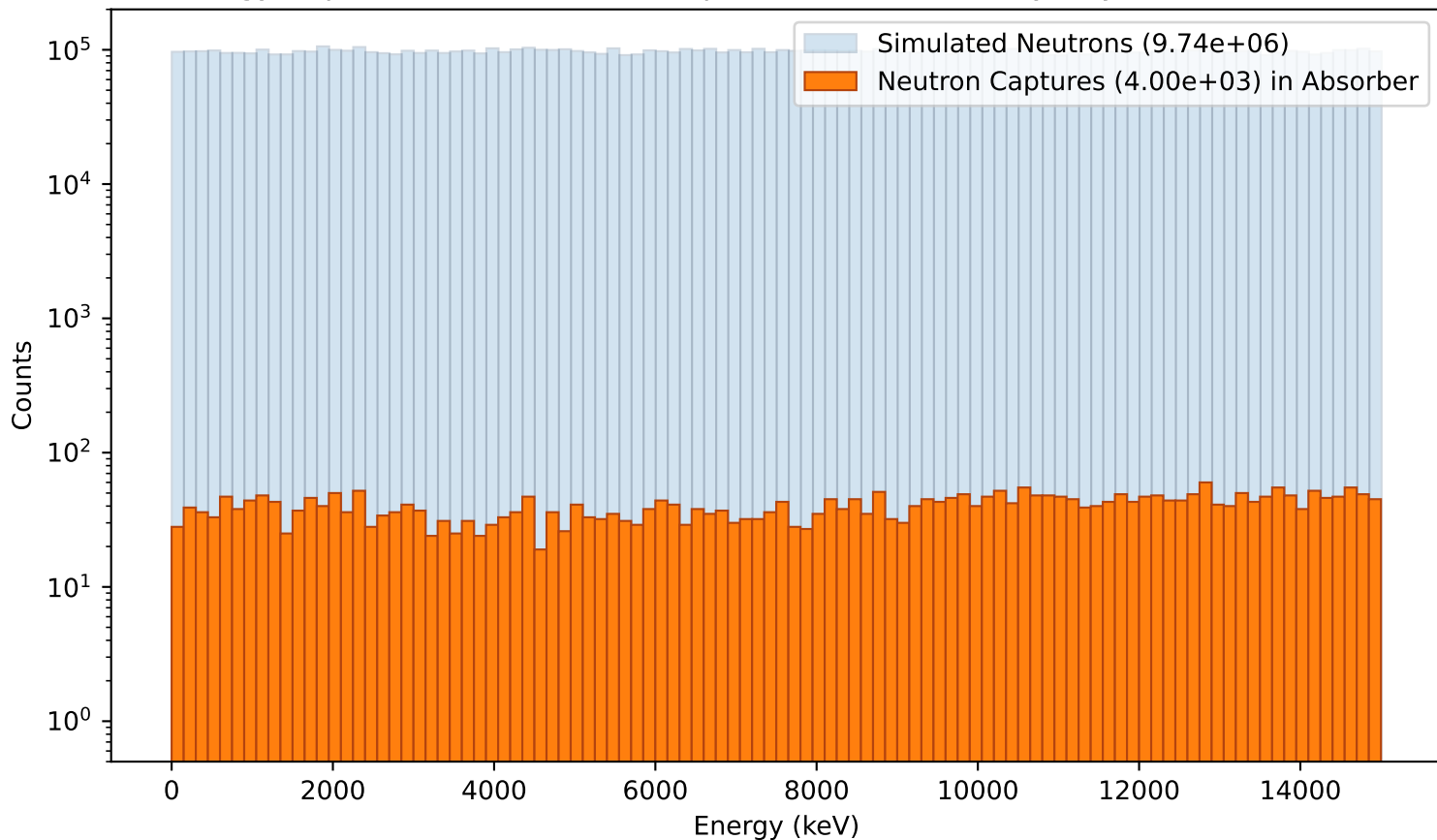
Energy dependence of Neutron Captures in the 5cm Polyethylene25 Absorber
