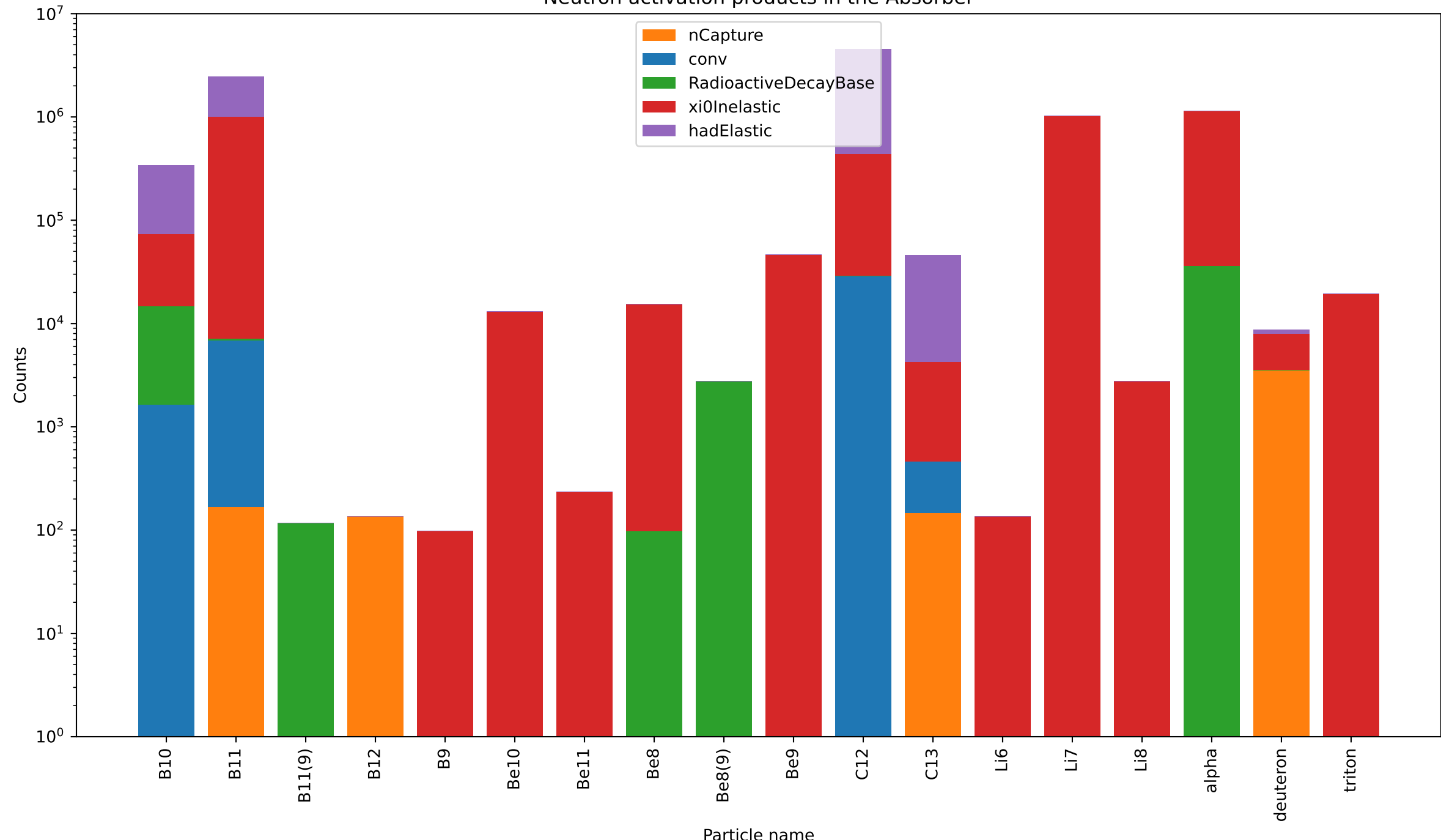
Neutron activation products in the Absorber
