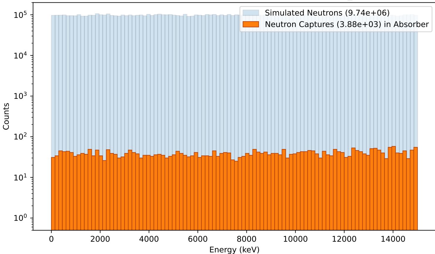
Energy dependence of Neutron Captures in the 5cm Polyethylene25_G4Boron Absorber
