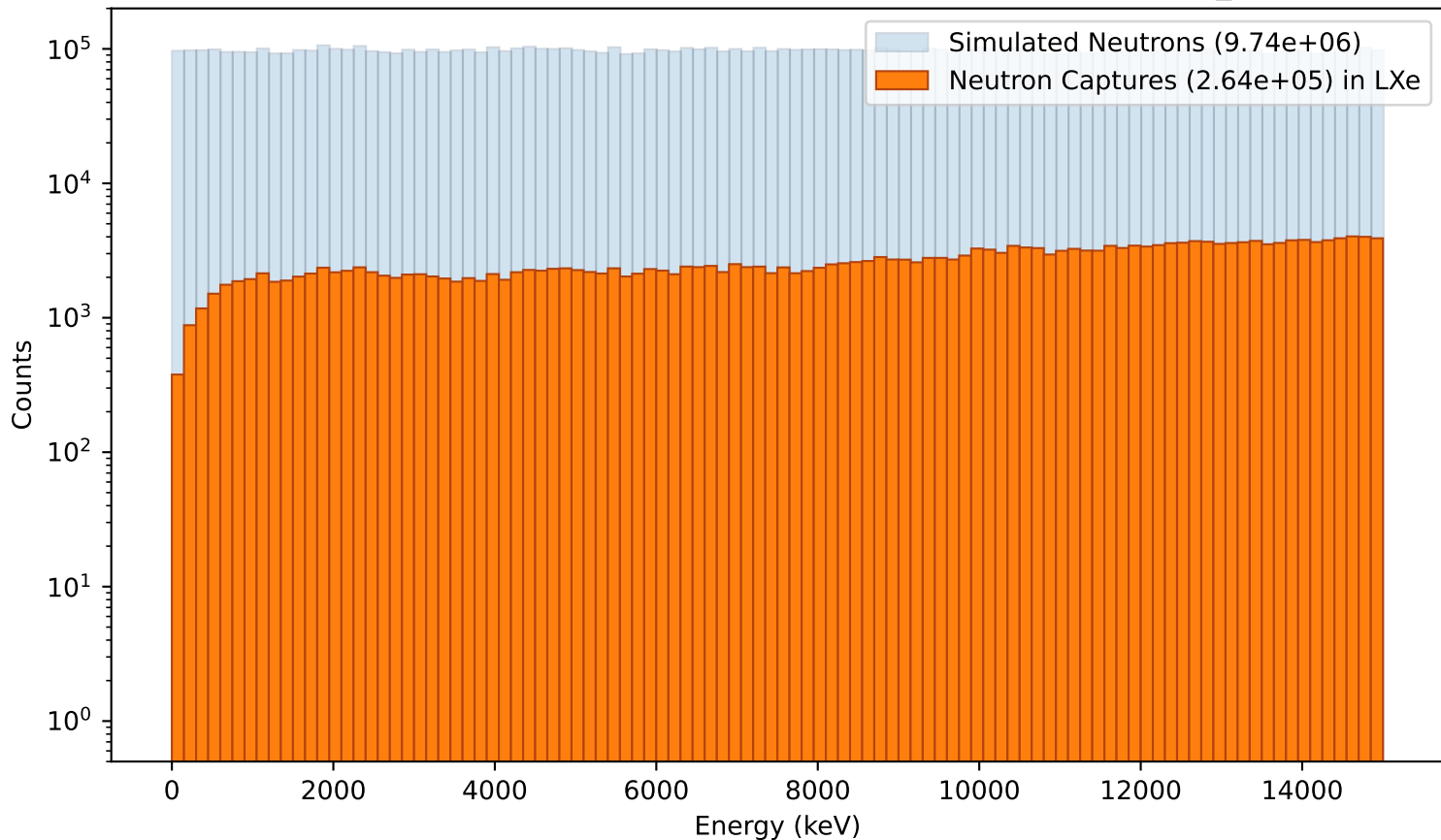
Energy dependence of Neutron Captures in LXe using a 5cm Polyethylene25_G4Boron Absorber
