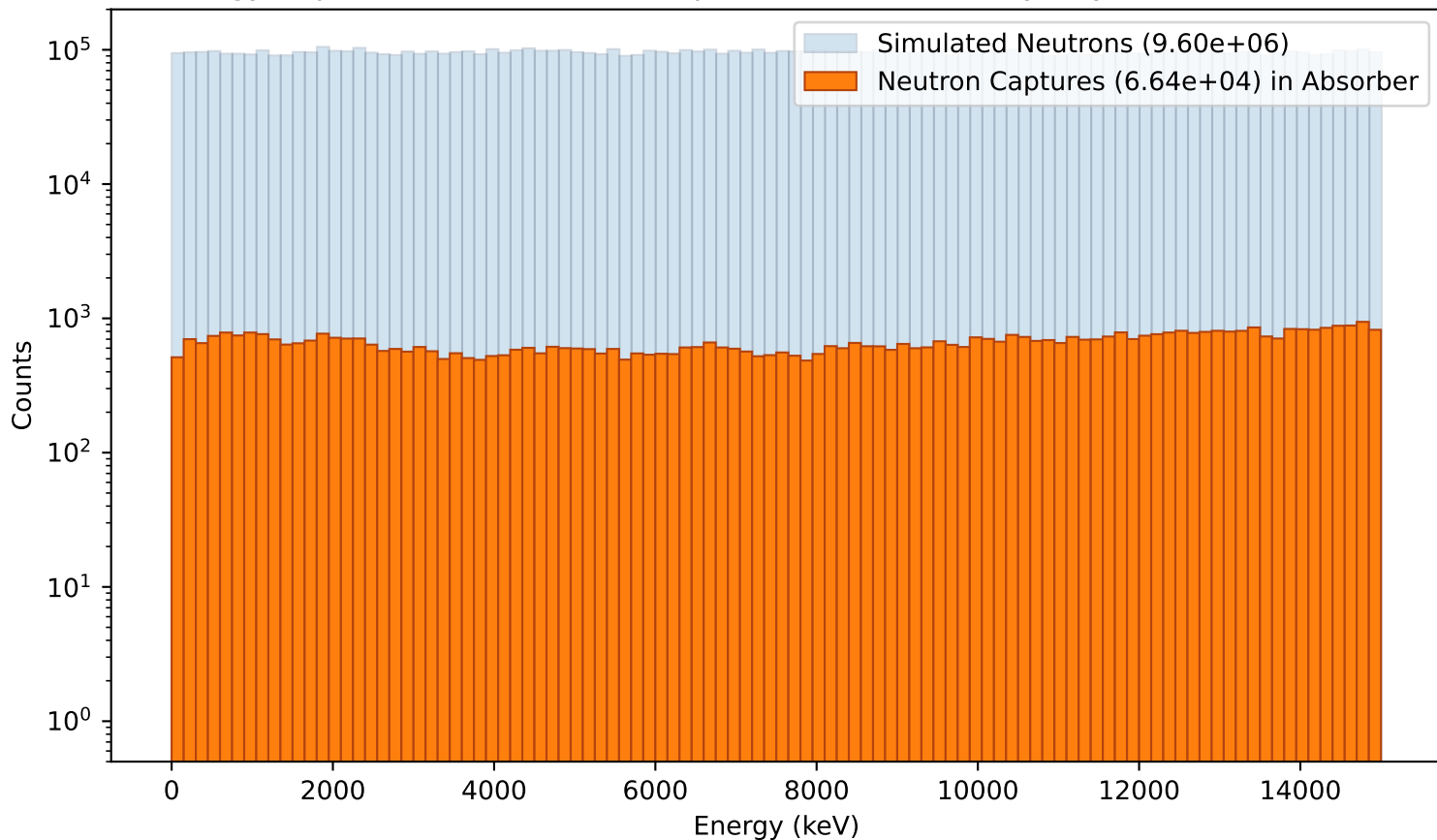
Energy dependence of Neutron Captures in the 5cm Polyethylene7Lit Absorber
