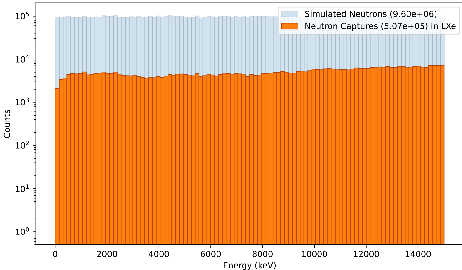
Energy dependence of Neutron Captures in LXe using a 5cm Polyethylene7Lit Absorber
