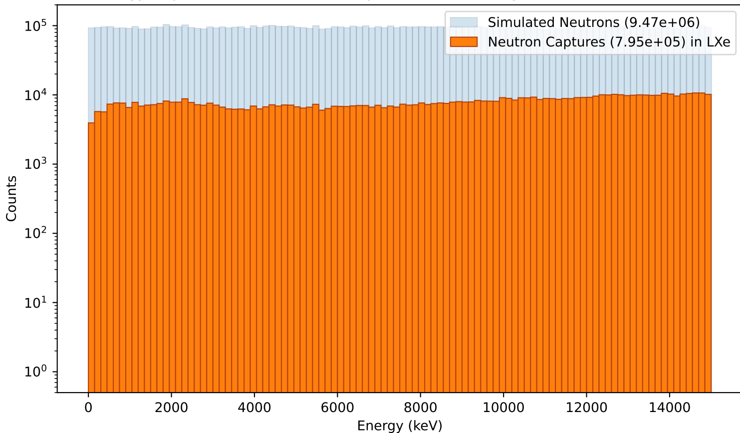
Energy dependence of Neutron Captures in LXe using a 5cm Water Absorber
