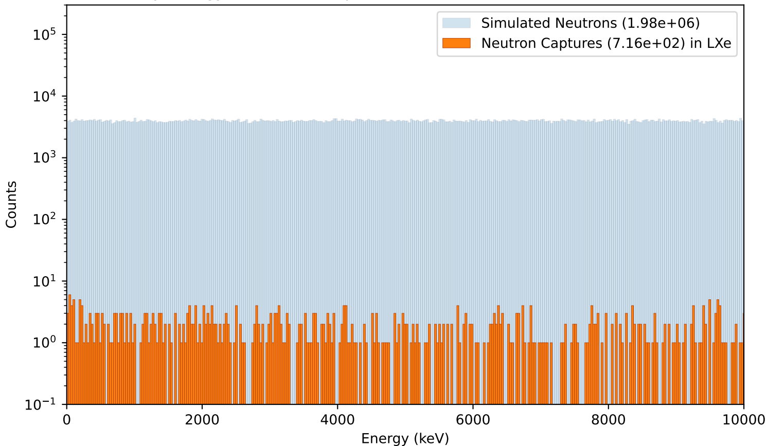
Primary energy of Neutron Captures in LXe (OneLXeVolumes,NoAbsorber)
