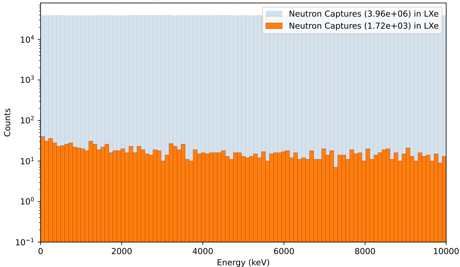
Primary energy of Neutron Captures in LXe (10cm,NoAbsorber)
