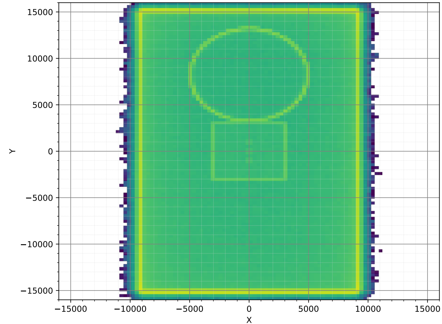
NeutronActivations (10cm, NoAbsorber, 4.88e+07)
