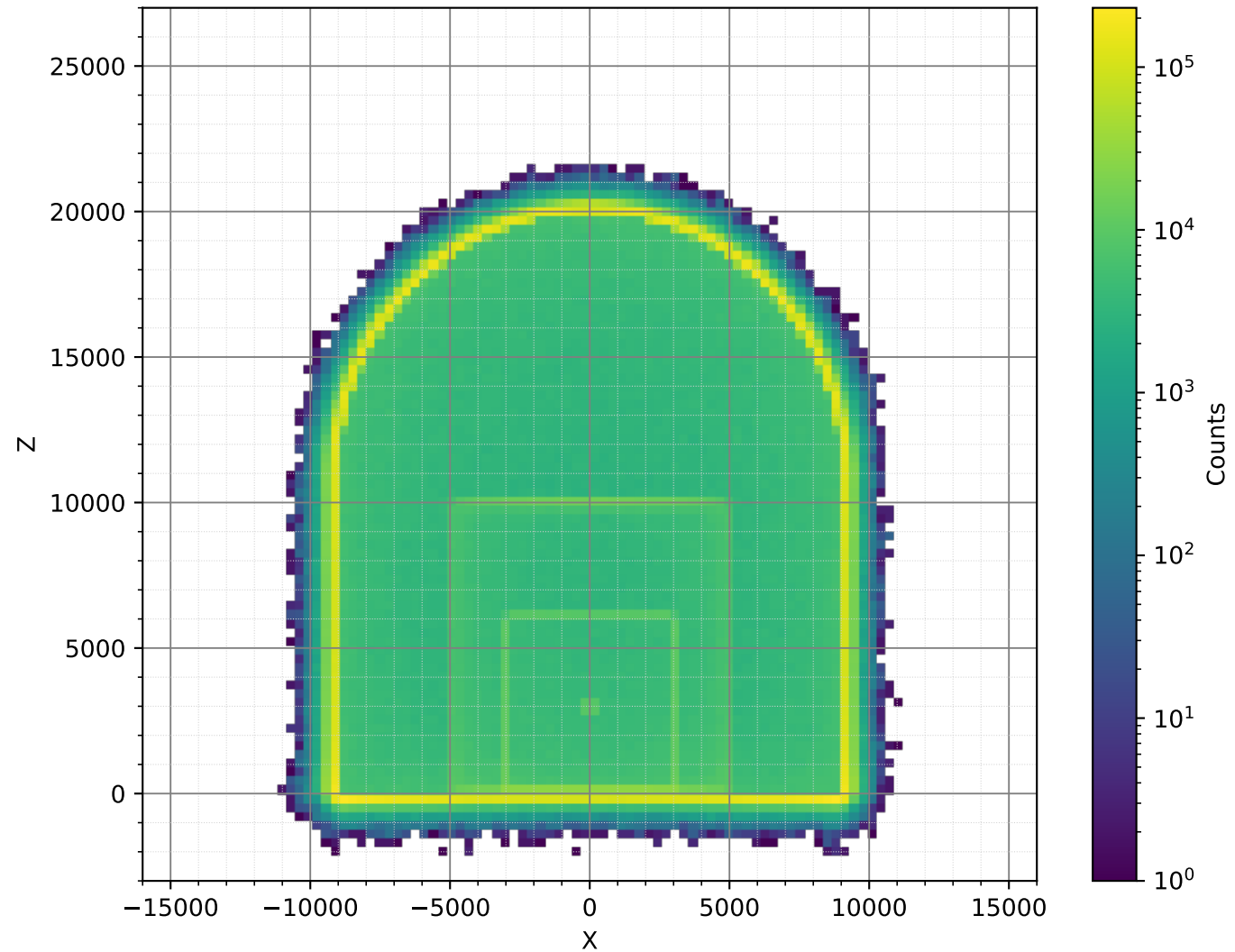
NeutronActivations (10cm, NoAbsorber, 4.88e+07)
