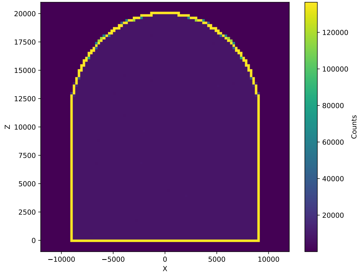
PrimaryNeutrons (10cm, NoAbsorber, 1.98e+08)
