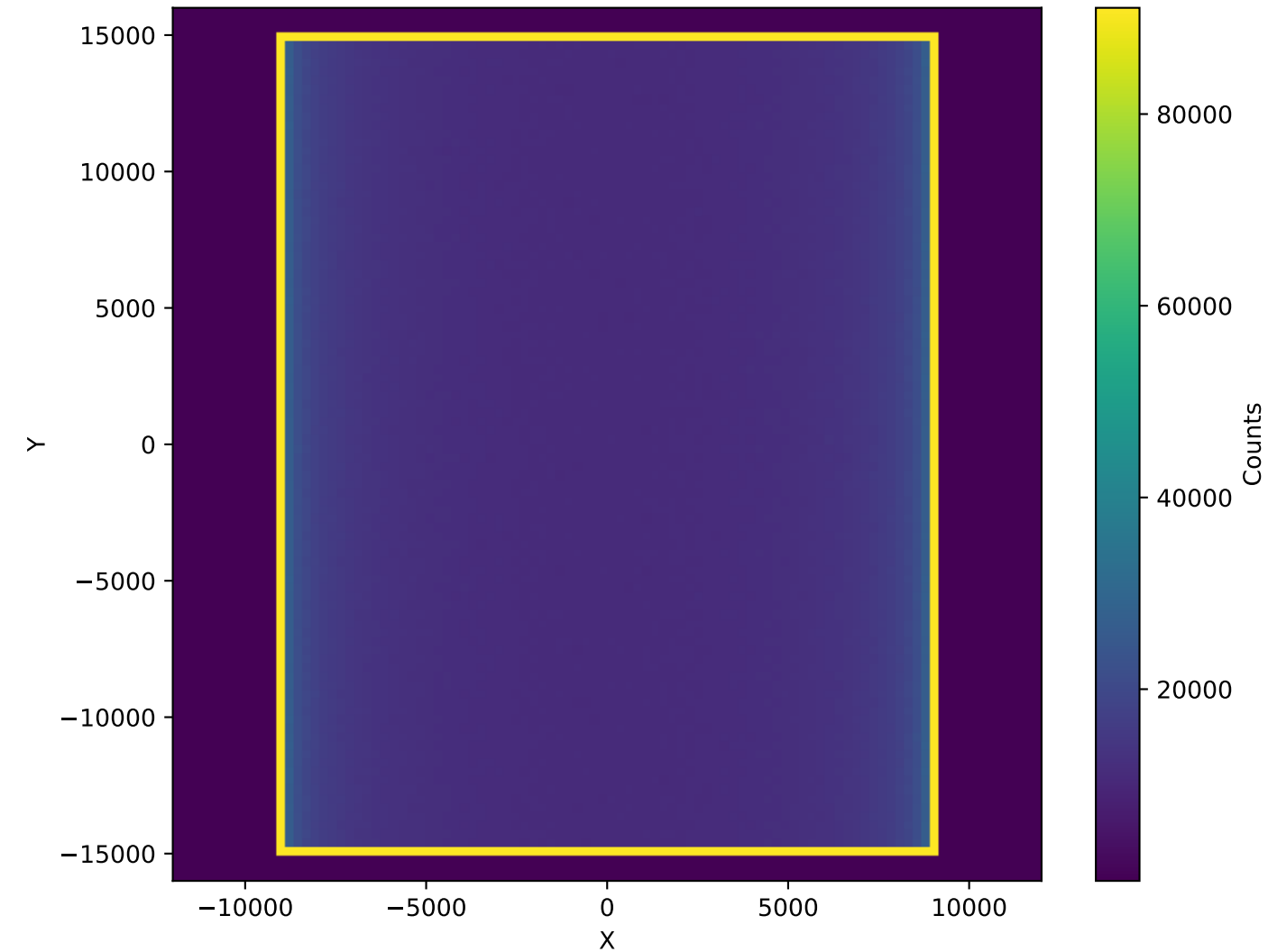
PrimaryNeutrons (10cm, NoAbsorber, 1.98e+08)
