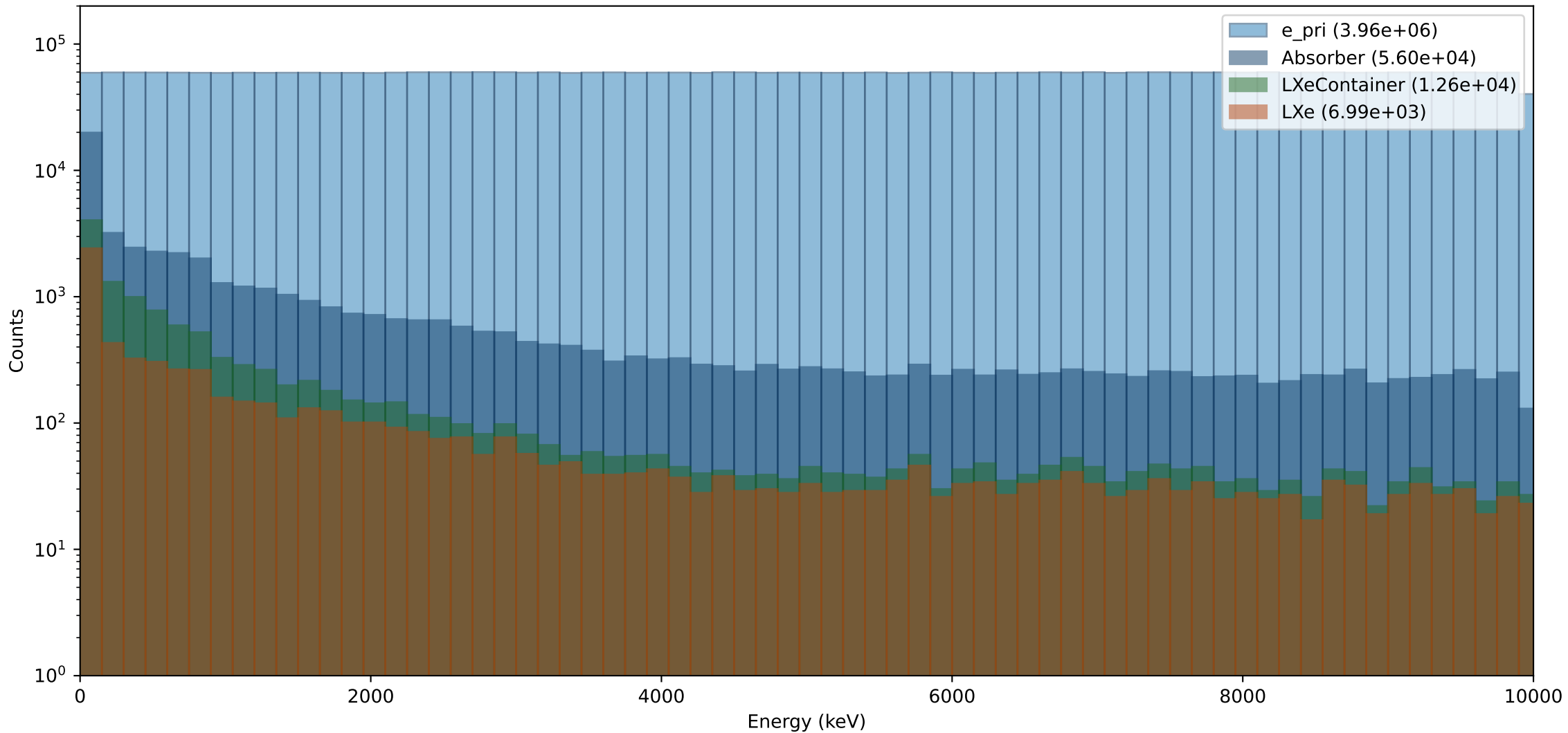
Energy distribution entering different volumes (50cm NoAbsorber)
