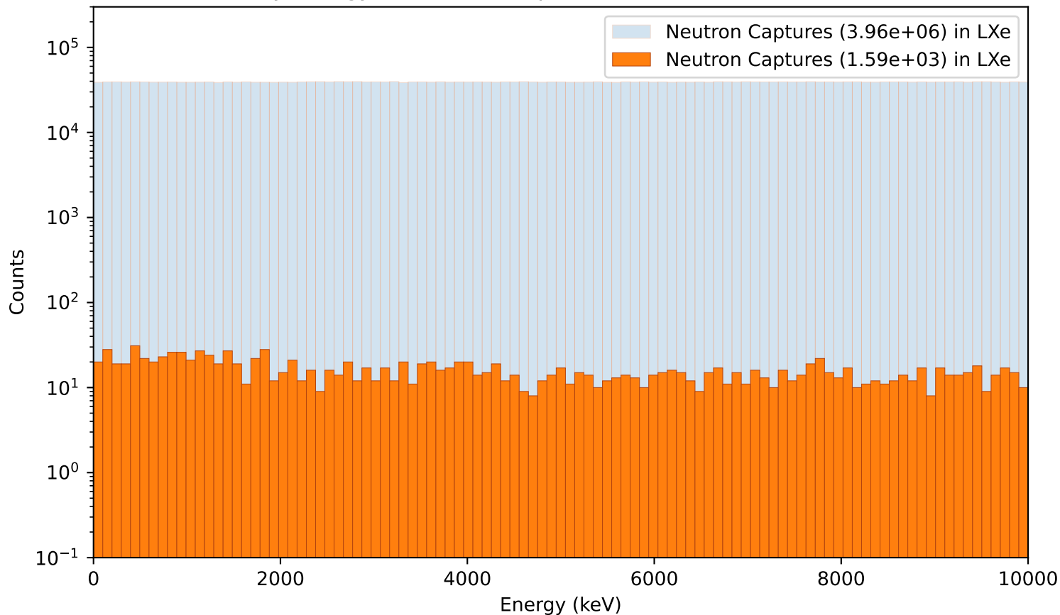
Primary energy of Neutron Captures in LXe (50cm,NoAbsorber)
