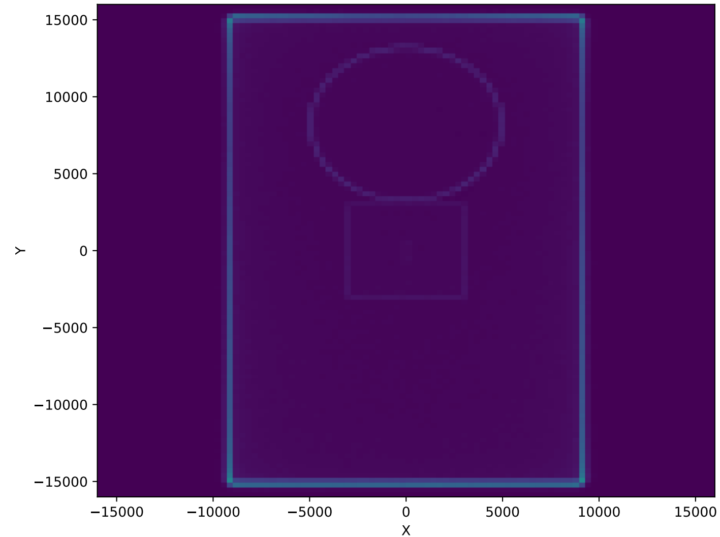
NeutronActivations (50cm, NoAbsorber)
