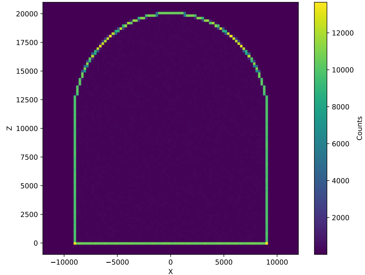
PrimaryNeutrons (50cm, NoAbsorber)
