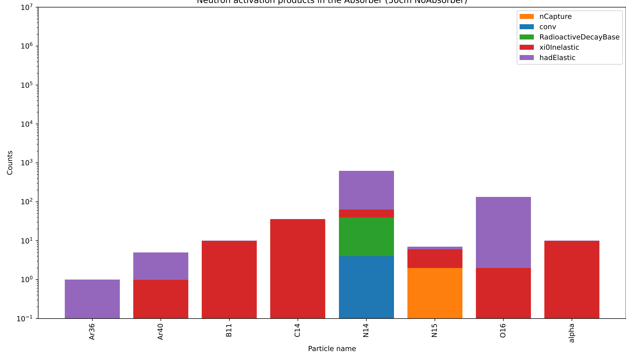
Neutron activation products in the Absorber (50cm NoAbsorber)
