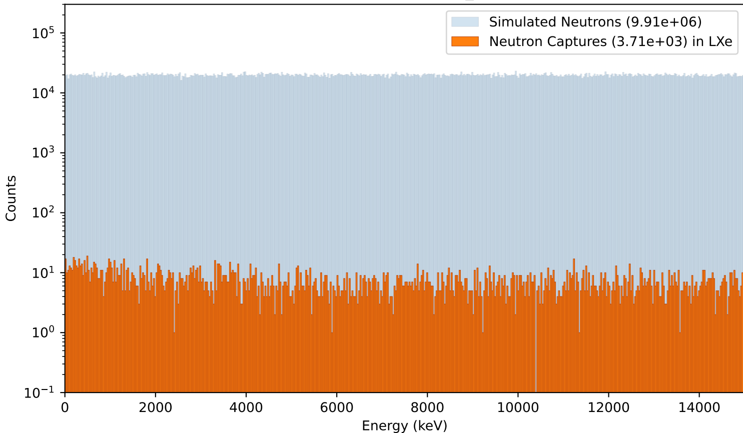
Primary energy of Neutron Captures in LXe (isoHalf_50cm,NoAbsorber,OneLXeVolumes)
