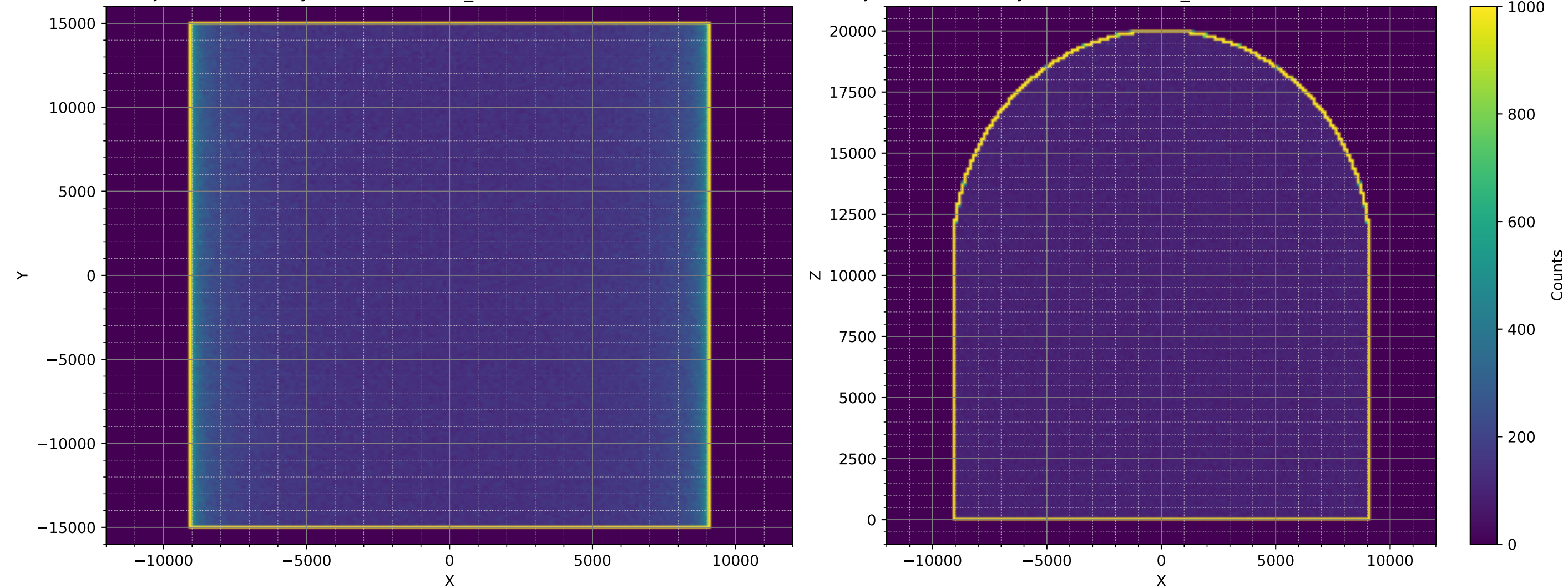
XY-Projection of PrimaryNeutrons (isoHalf_50cm, NoAbsorber, OneLXeVolumes) XZ-Projection of PrimaryNeutrons (isoHalf_50cm, NoAbsorber, OneLXeVolumes)
