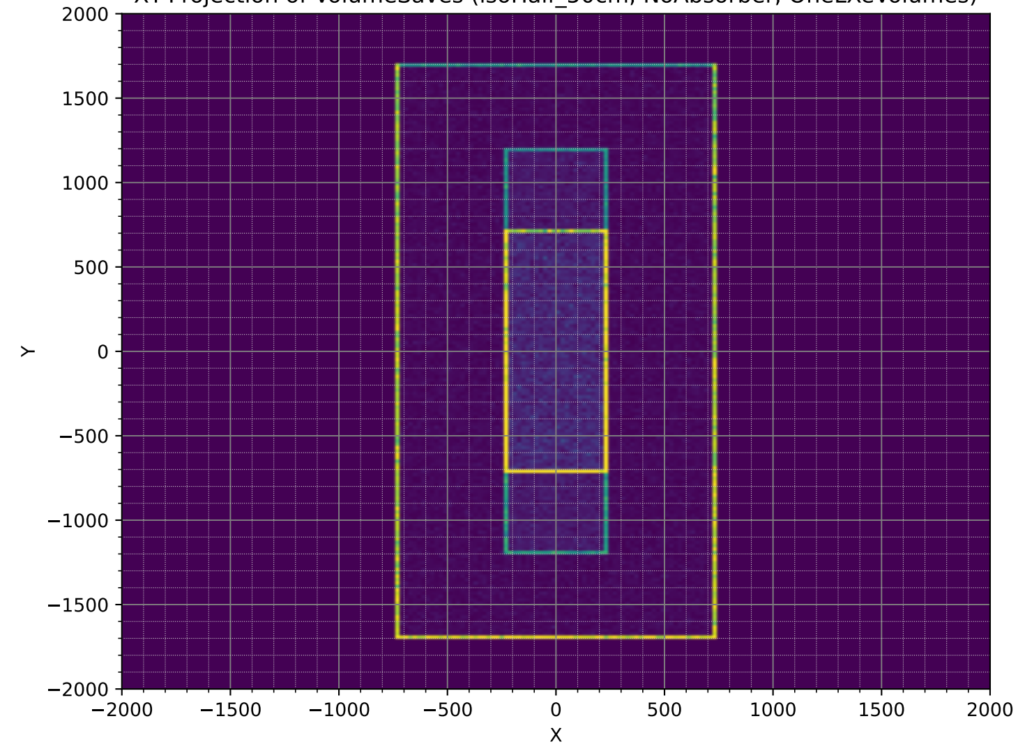
XY-Projection of VolumeSaves (isoHalf_50cm, NoAbsorber, OneLXeVolumes)
