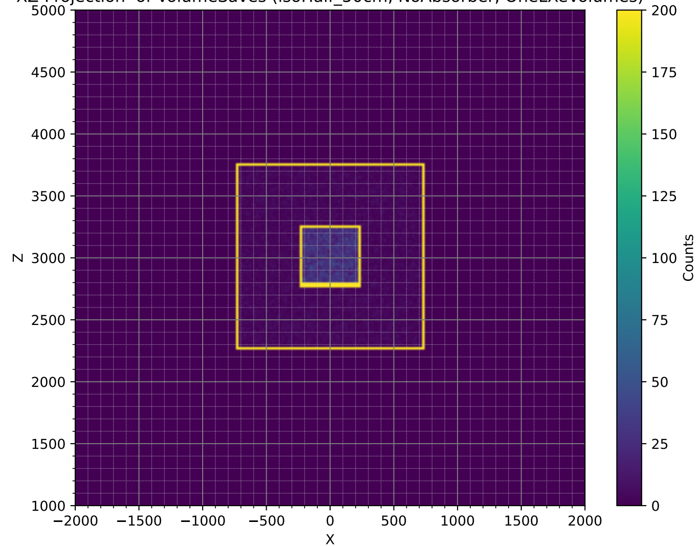
XZ-Projection of VolumeSaves (isoHalf_50cm, NoAbsorber, OneLXeVolumes)
