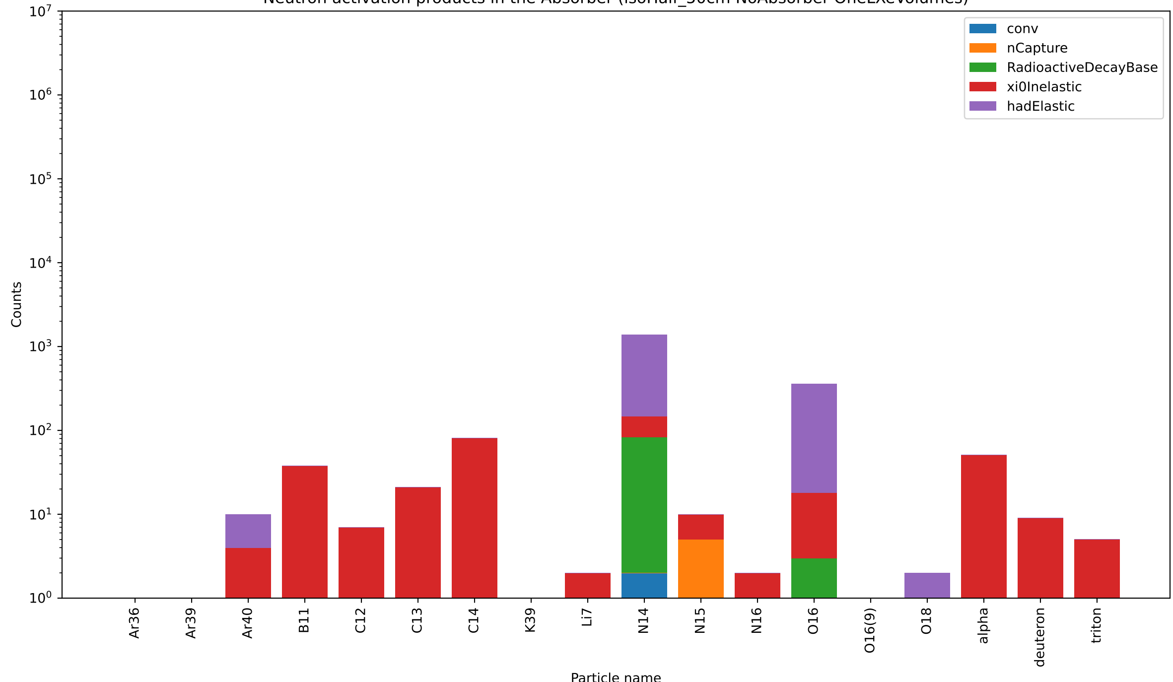
Neutron activation products in the Absorber (isoHalf_50cm NoAbsorber OneLXeVolumes)
