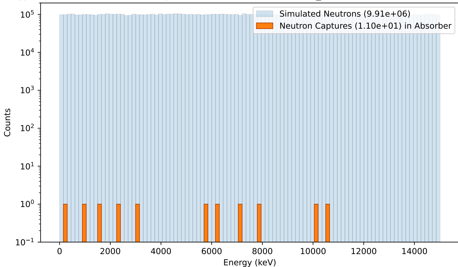
Energy dependence of Neutron Captures in the Absorber (isoHalf_50cm,NoAbsorber,ThreeLXeV
