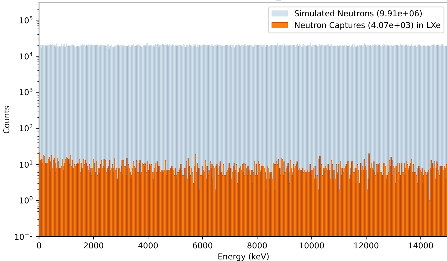
Primary energy of Neutron Captures in LXe (isoHalf_50cm,NoAbsorber,ThreeLXeVolumes)
