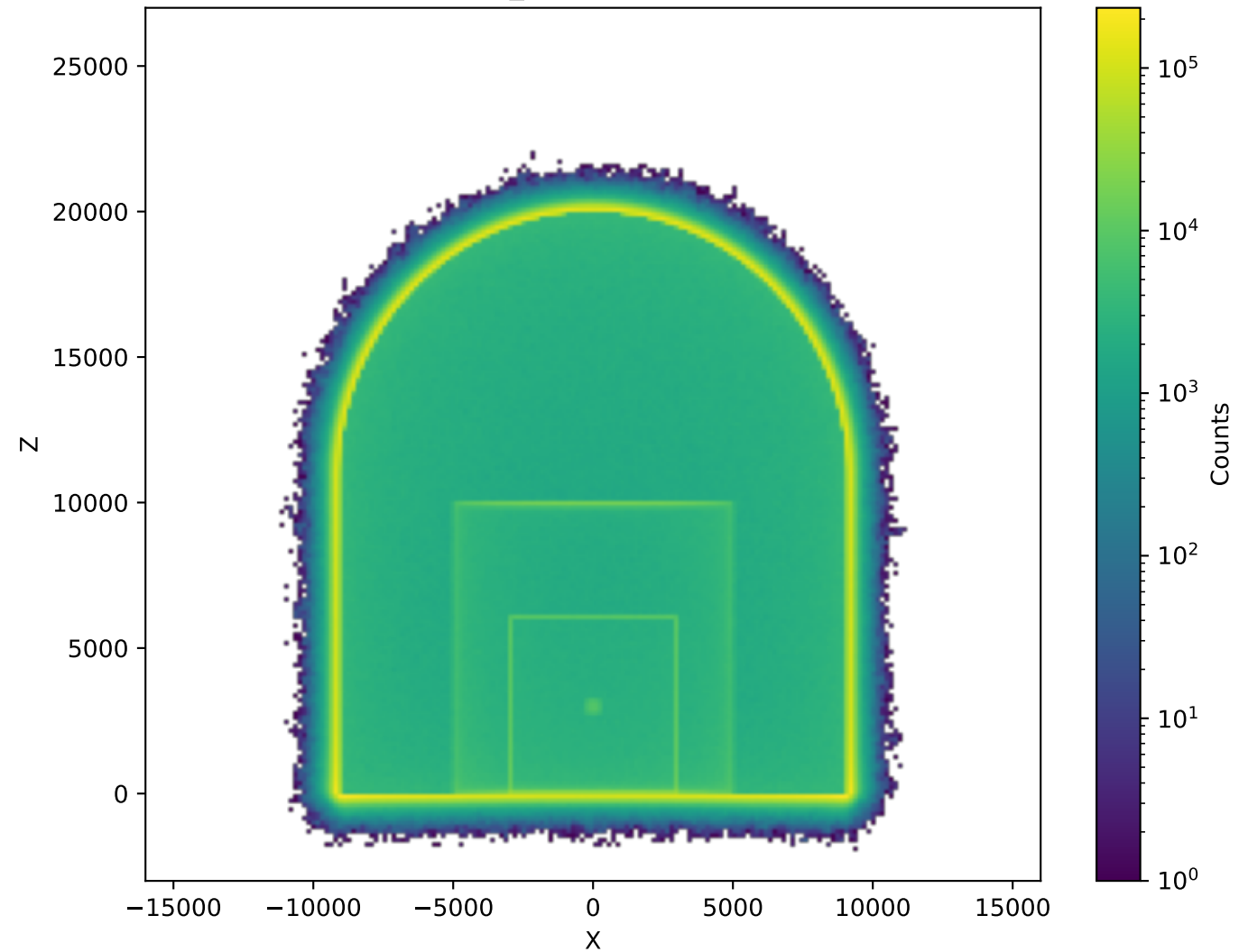
NeutronActivations (isoHalf_50cm, NoAbsorber, ThreeLXeVolumes)
