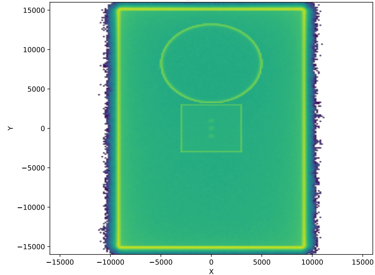
NeutronActivations (isoHalf_50cm, NoAbsorber, ThreeLXeVolumes)
