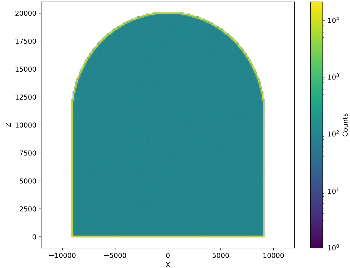
PrimaryNeutrons (isoHalf_50cm, NoAbsorber, ThreeLXeVolumes)
