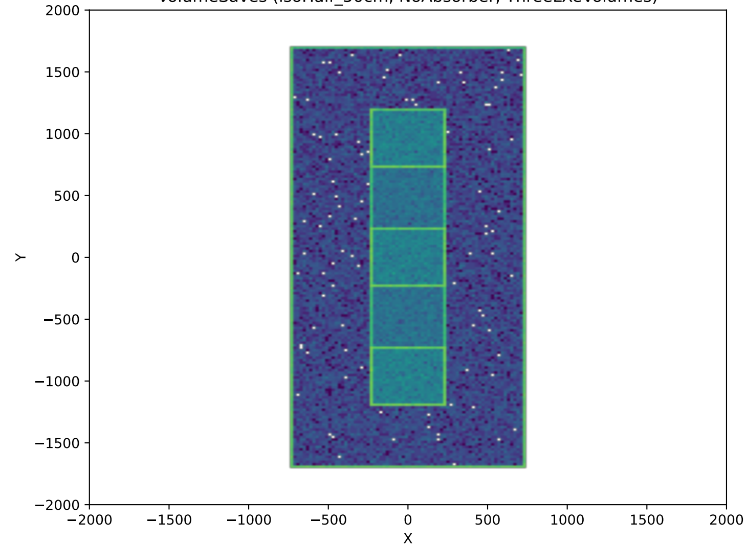
VolumeSaves (isoHalf_50cm, NoAbsorber, ThreeLXeVolumes)
