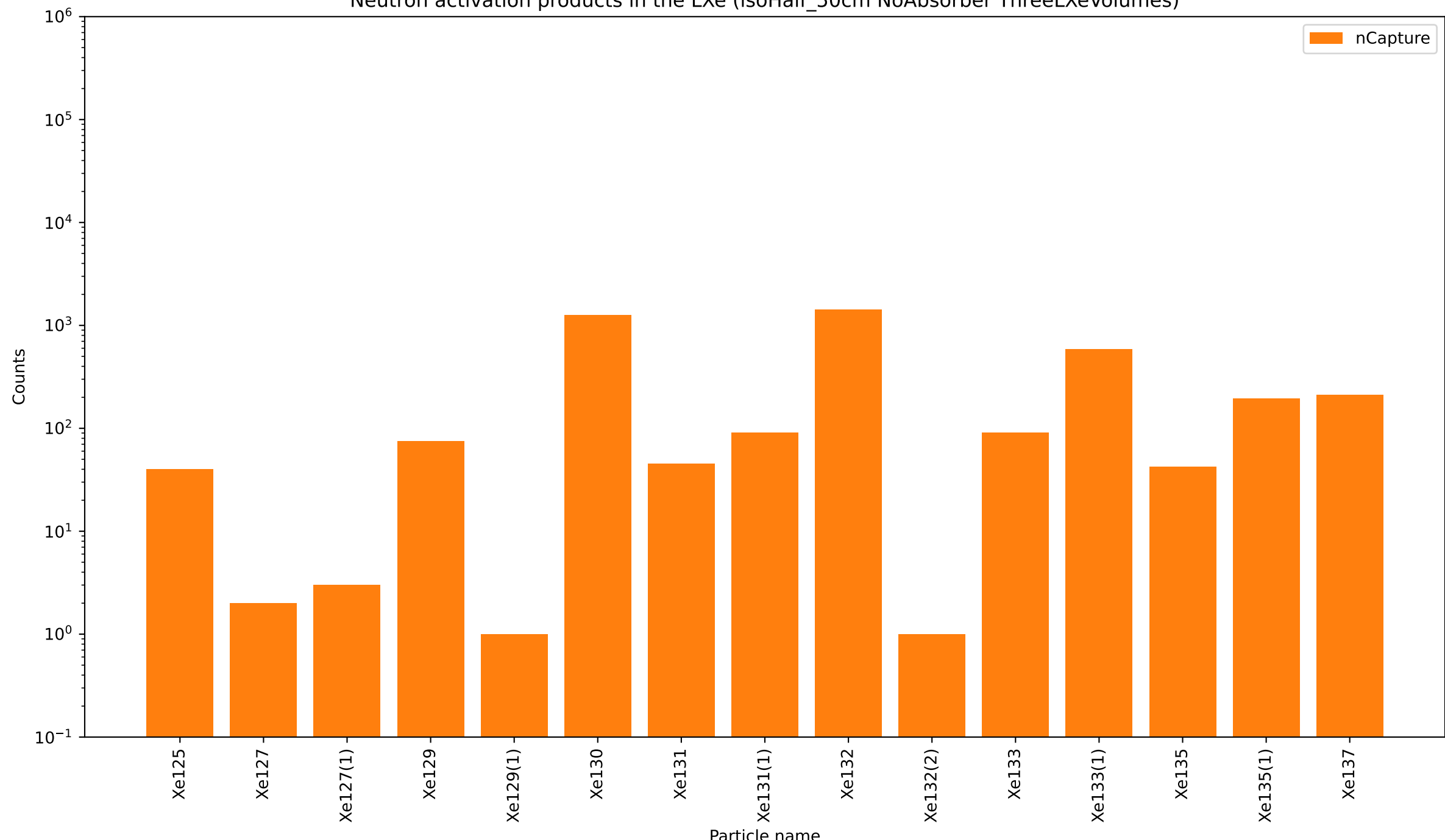
Neutron activation products in the LXe (isoHalf_50cm NoAbsorber ThreeLXeVolumes)
