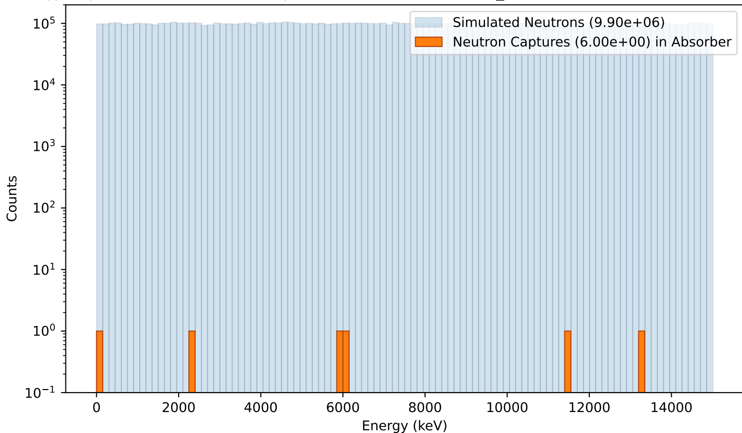
Energy dependence of Neutron Captures in the Absorber (iso_50cm,NoAbsorber,ThreeLXeVols)
