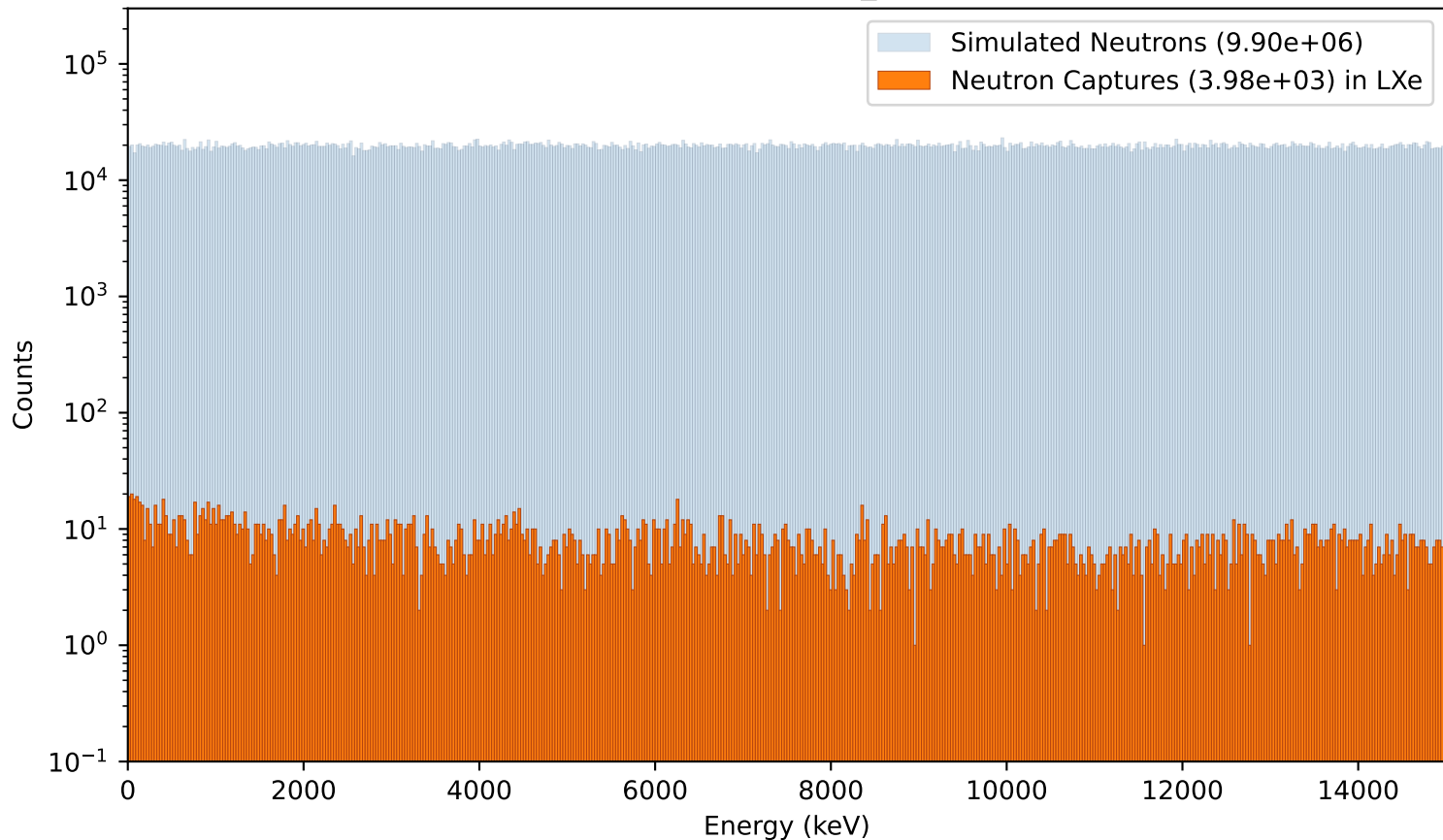
Primary energy of Neutron Captures in LXe (iso_50cm,NoAbsorber,ThreeLXeVolumes)
