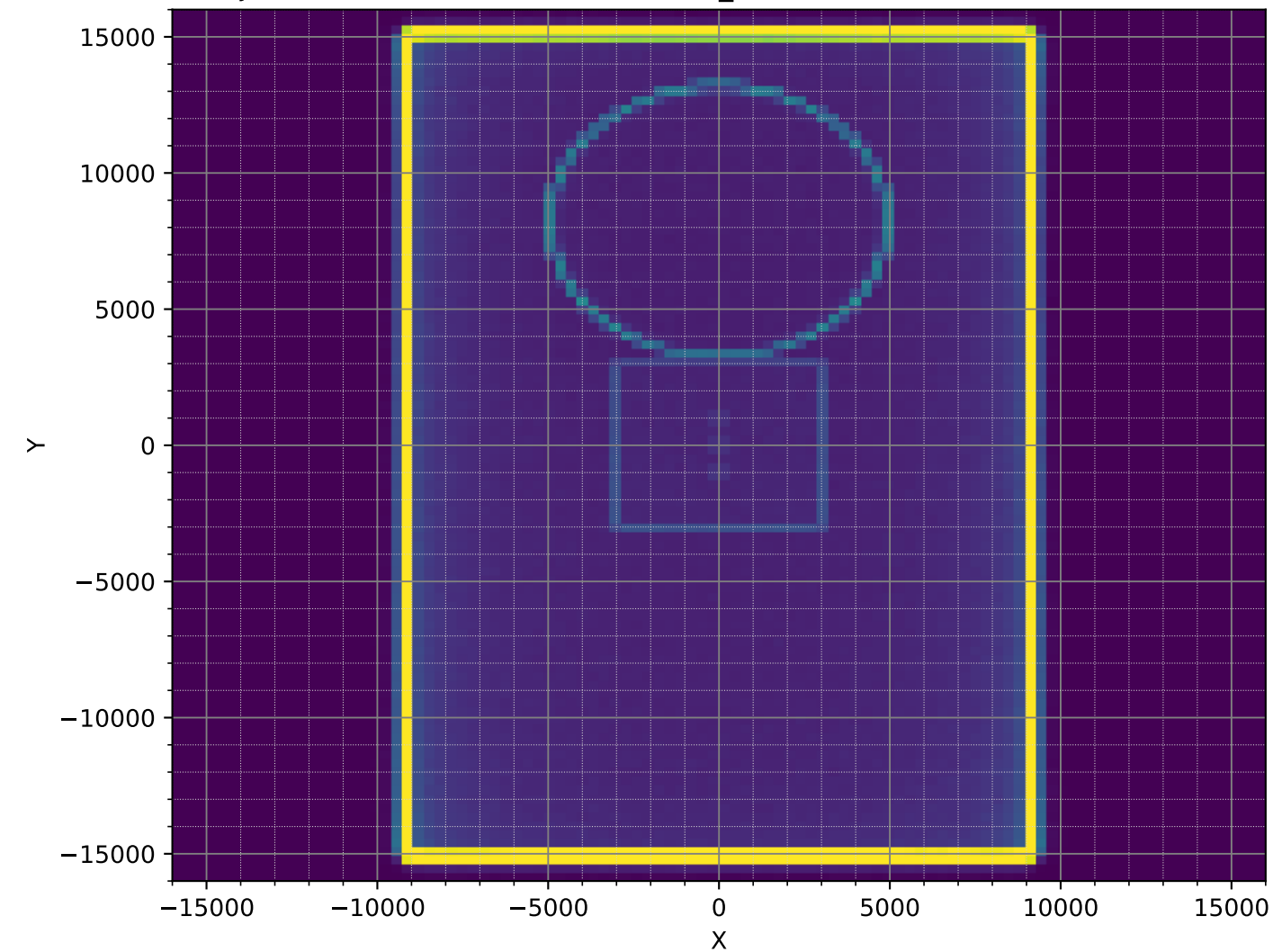
XY-Projection of NeutronActivations (iso_50cm, NoAbsorber, ThreeLXeVolumes)XZ-Projection of NeutronActivations (iso_50cm, NoAbsorber, ThreeLXeVolumes)
