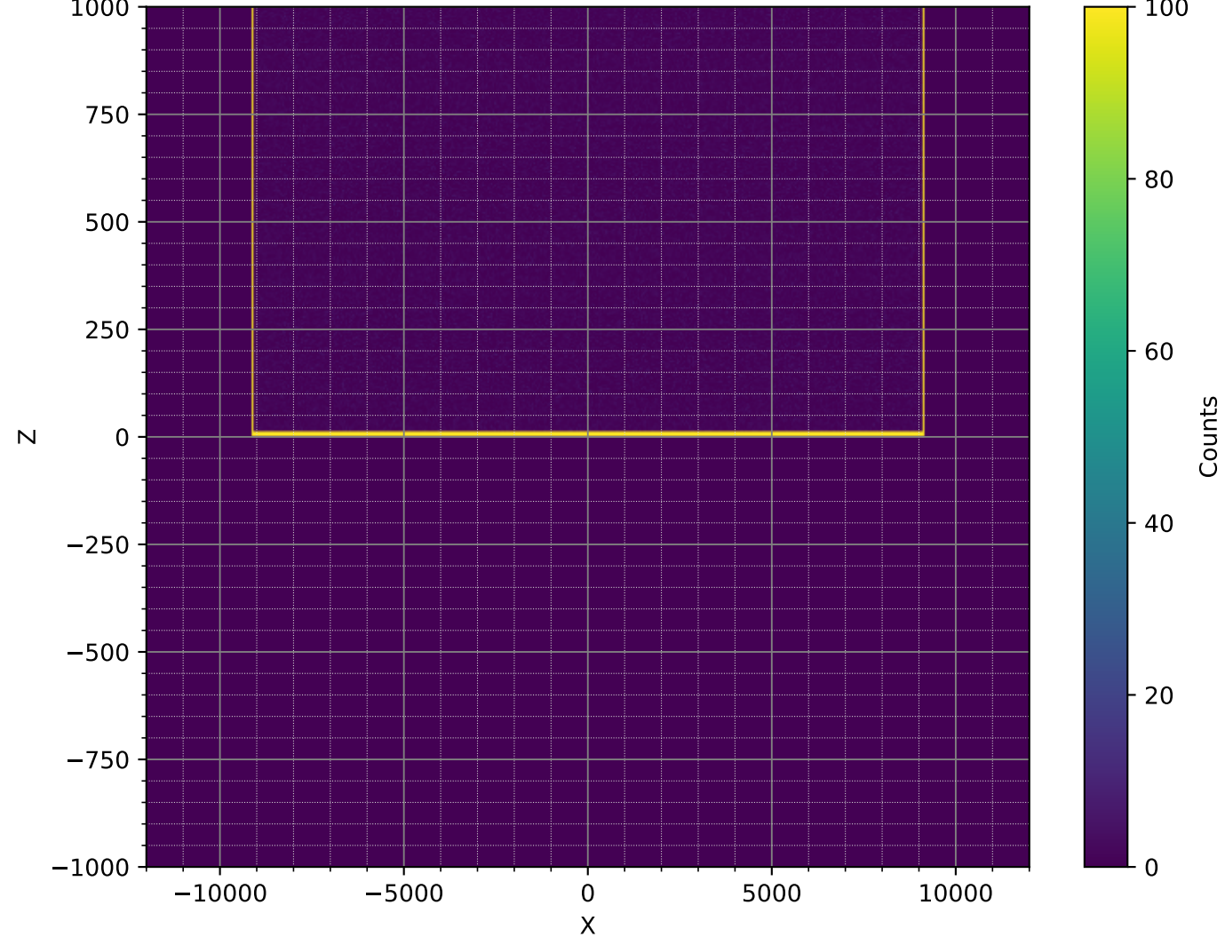
XZ-Projection of PrimaryNeutrons (iso_50cm, NoAbsorber, ThreeLXeVolumes)
