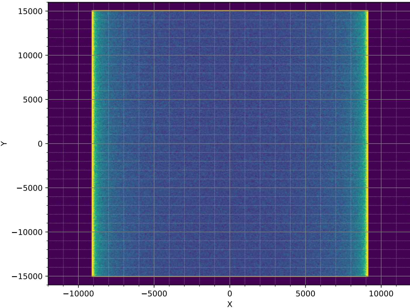
XY-Projection of PrimaryNeutrons (iso_50cm, NoAbsorber, ThreeLXeVolumes)
