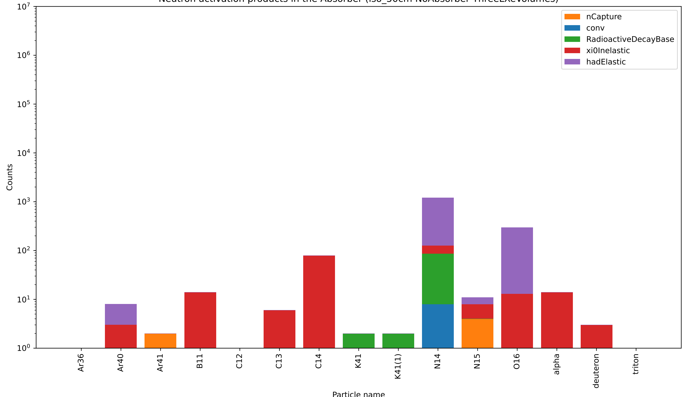
Neutron activation products in the Absorber (iso_50cm NoAbsorber ThreeLXeVolumes)
