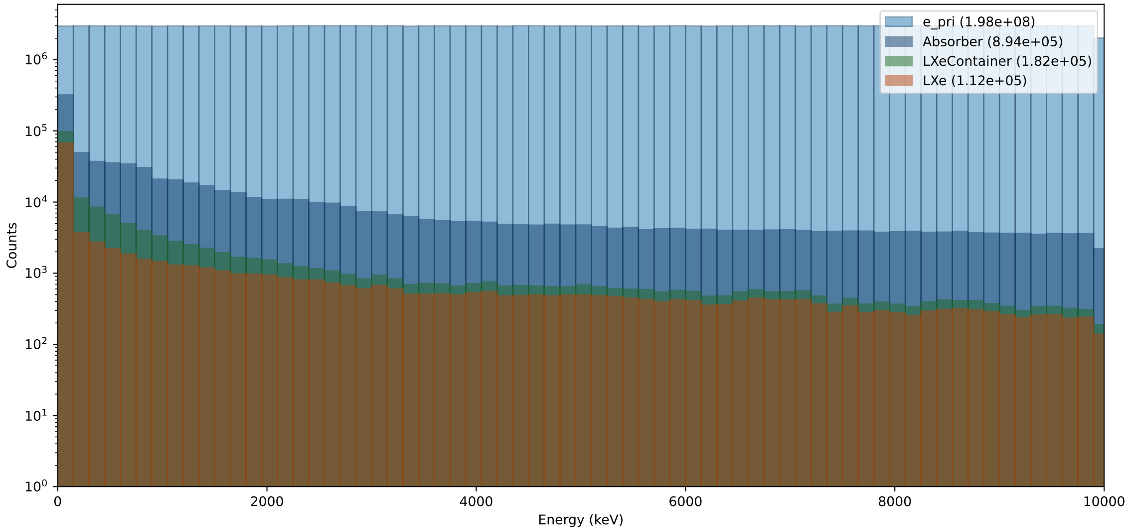
Energy distribution entering different volumes (10cm Polyethylen)
