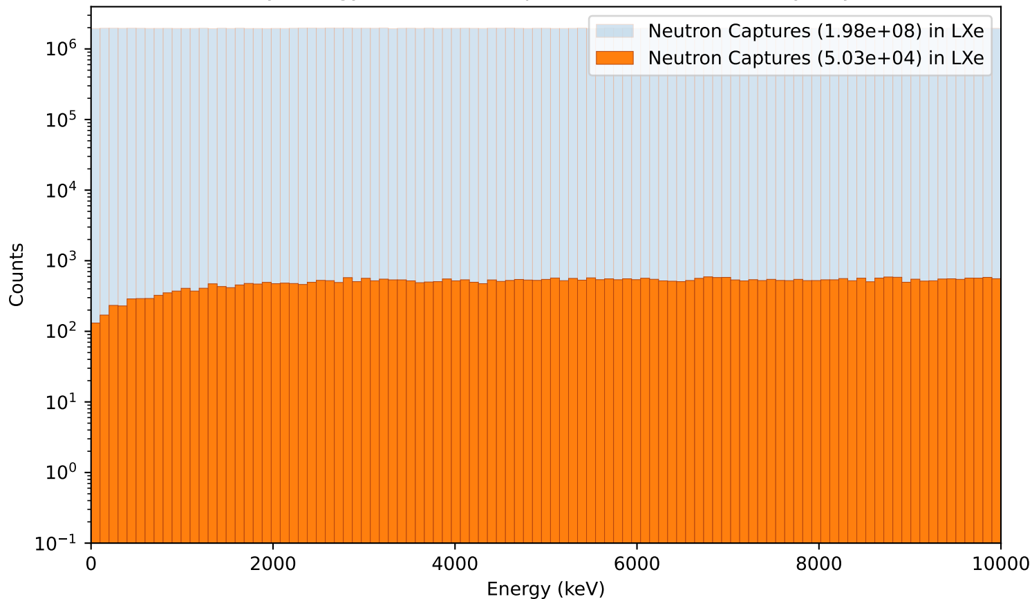
Primary energy of Neutron Captures in LXe (10cm,Polyethylen)
