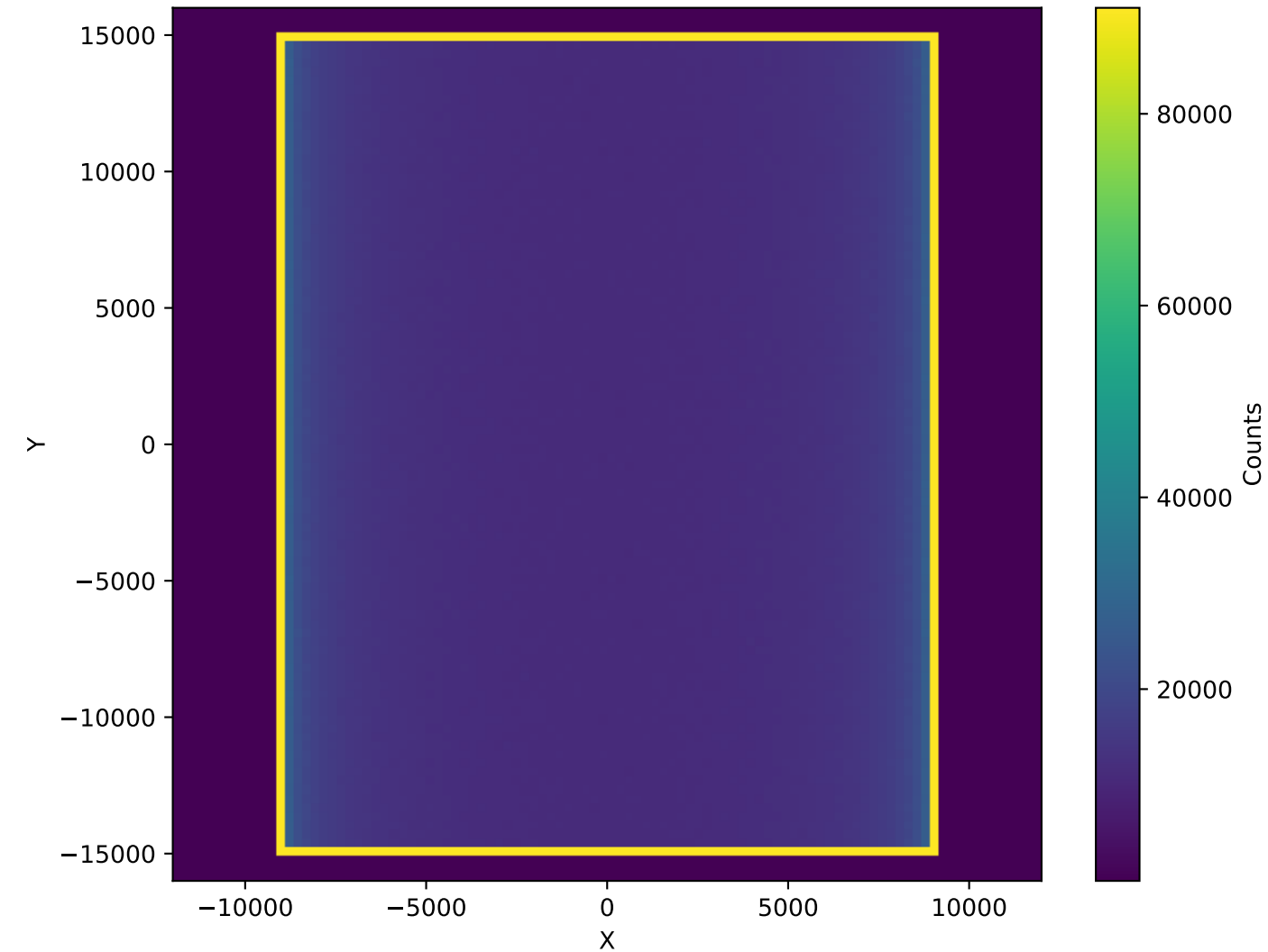
PrimaryNeutrons (10cm, Polyethylen, 1.98e+08)
