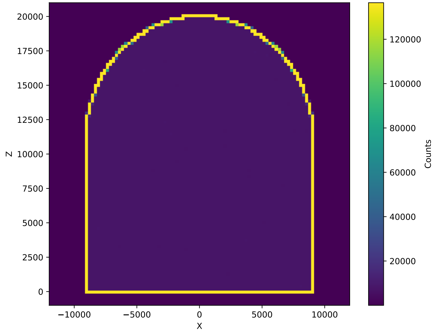
PrimaryNeutrons (10cm, Polyethylen, 1.98e+08)
