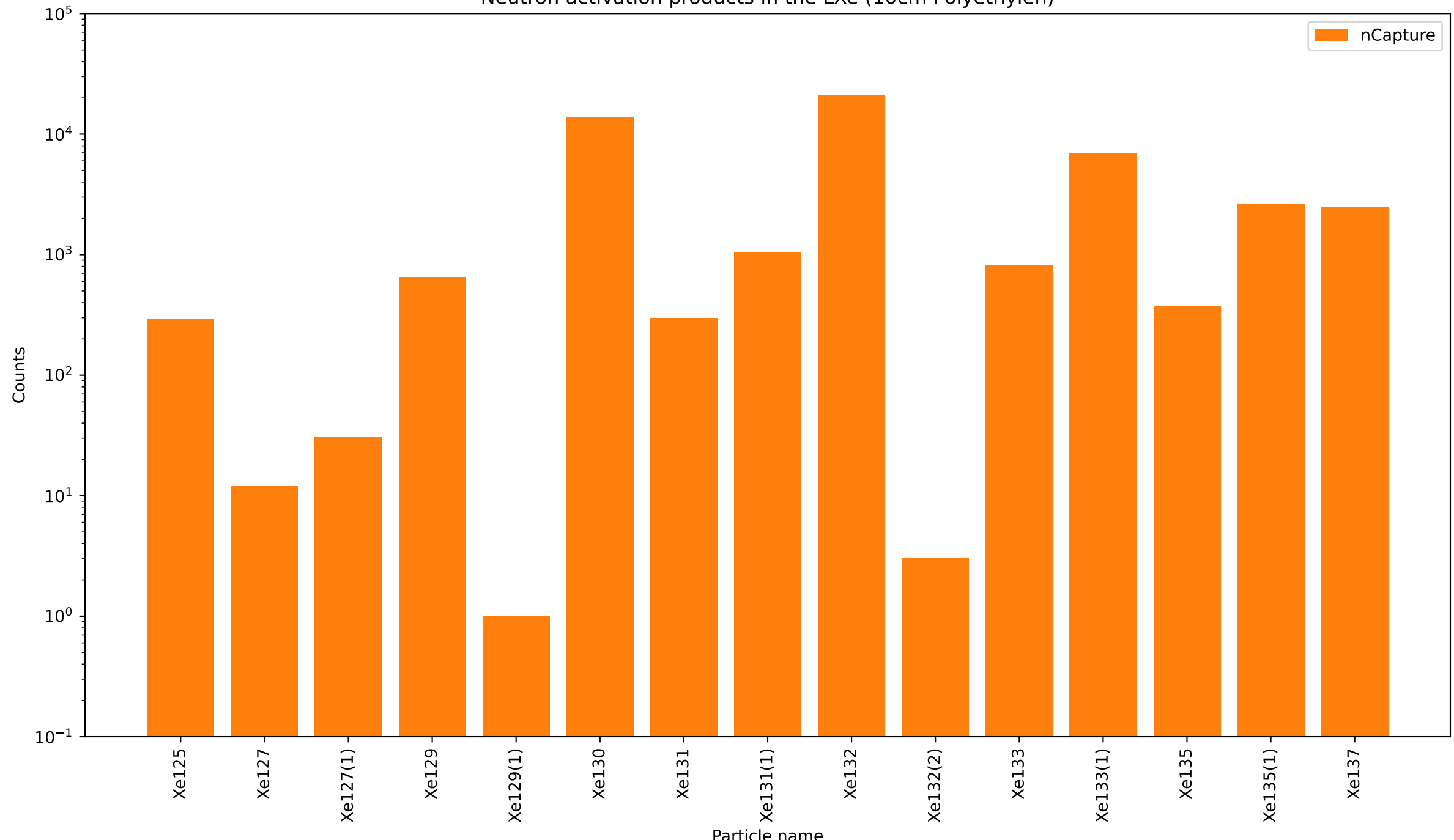
Neutron activation products in the LXe (10cm Polyethylen)
