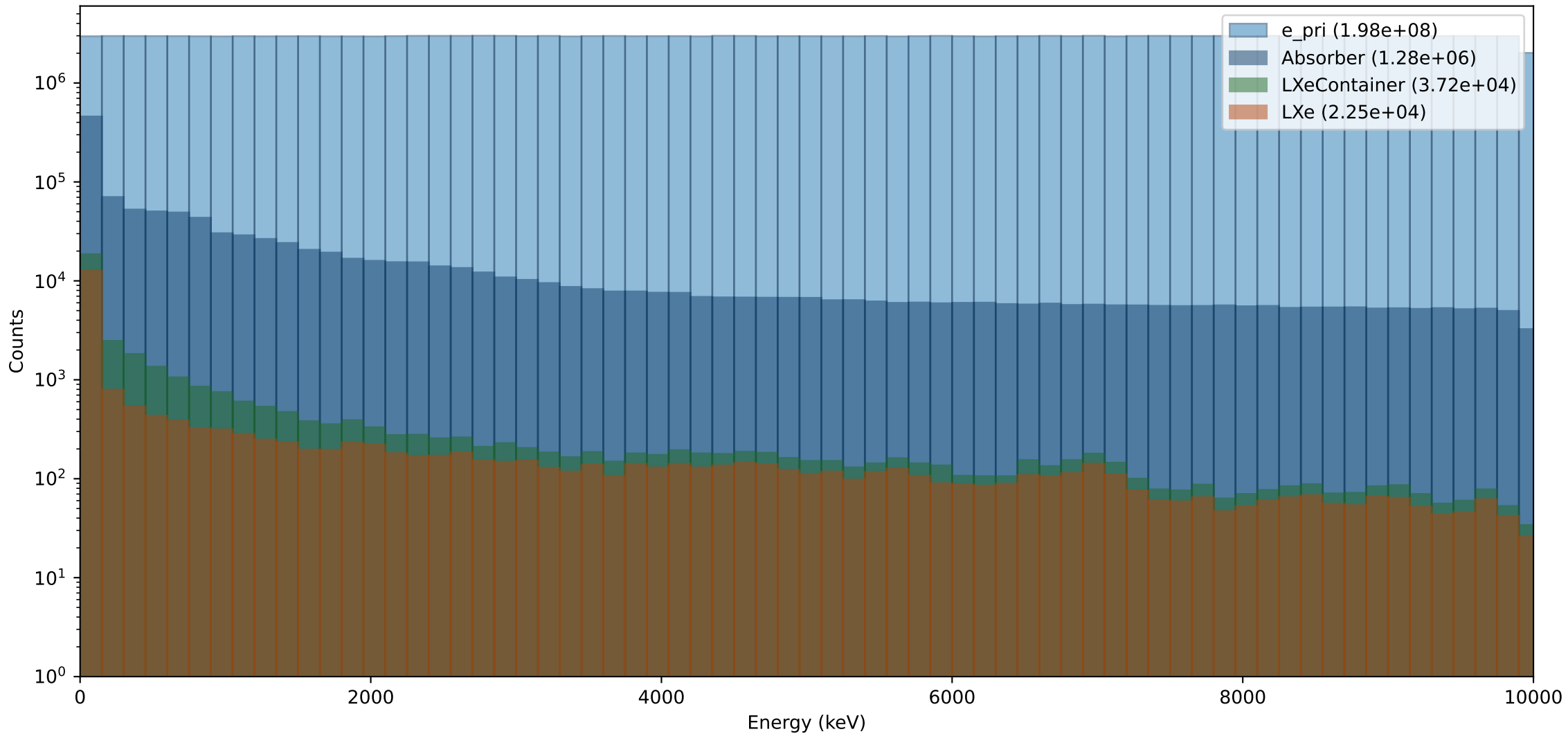
Energy distribution entering different volumes (20cm Polyethylen)
