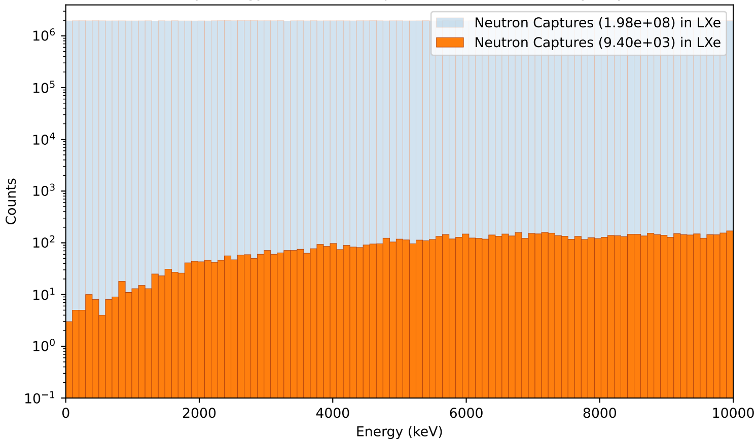
Primary energy of Neutron Captures in LXe (20cm,Polyethylen)
