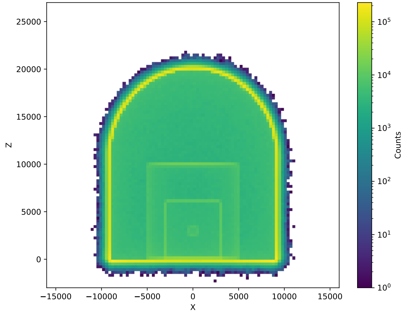
NeutronActivations (20cm, Polyethylen)
