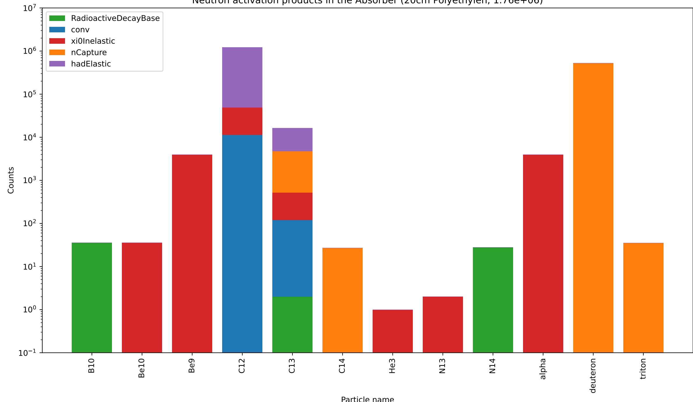
Neutron activation products in the Absorber (20cm Polyethylen, 1.76e+06)
