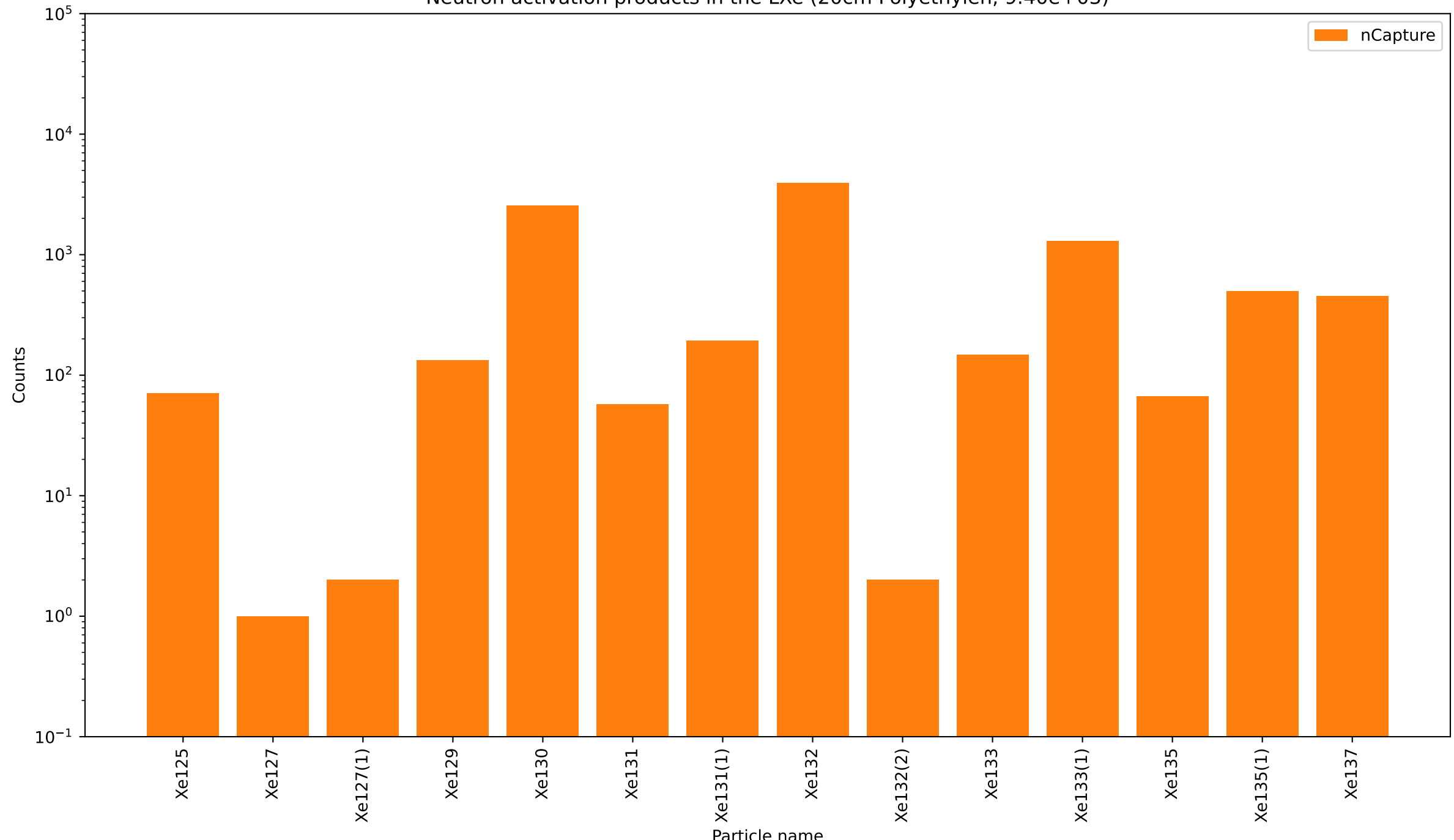
Neutron activation products in the LXe (20cm Polyethylen, 9.40e+03)
