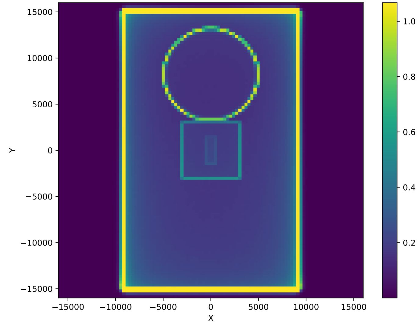
NeutronActivations (30cm, Polyethylen, 2.43e+09)
