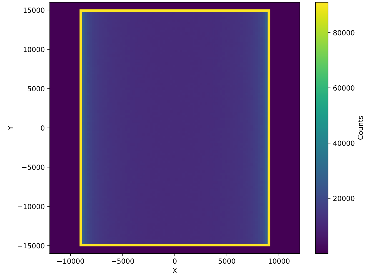
PrimaryNeutrons (30cm, Polyethylen, 1.98e+08)
