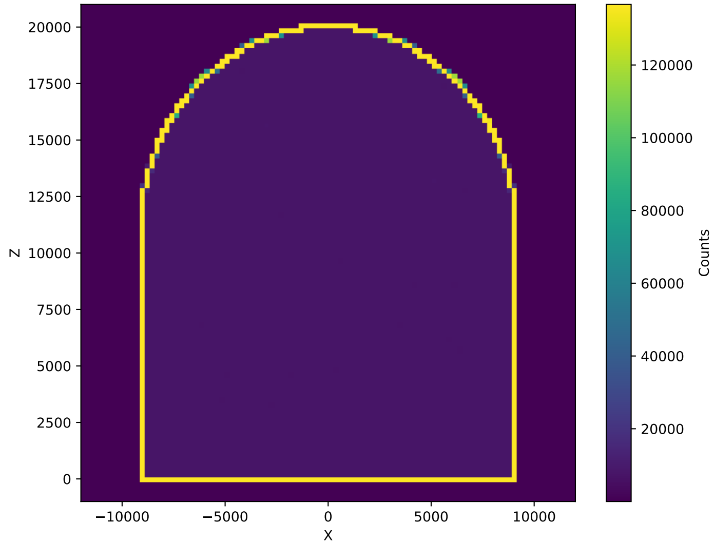
PrimaryNeutrons (30cm, Polyethylen, 1.98e+08)
