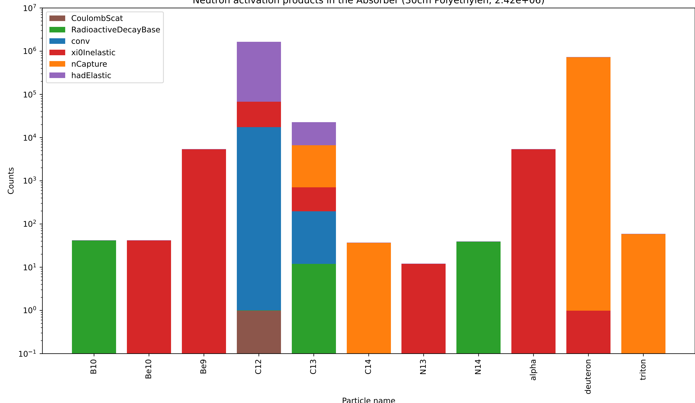
Neutron activation products in the Absorber (30cm Polyethylen, 2.42e+06)
